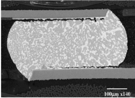
Figure 1: Crack Propagation at the Top and Bottom of a Solder Joint, 15mm BGA [2]
